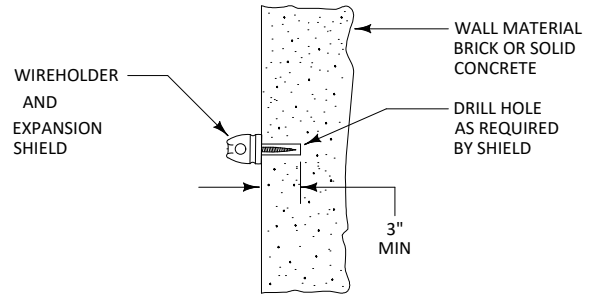
MASONRY
