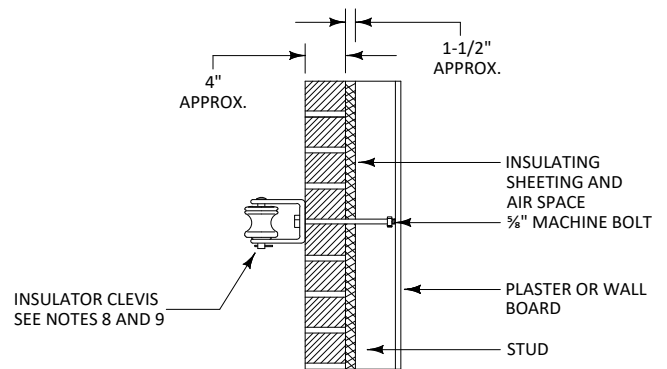
BRICK
