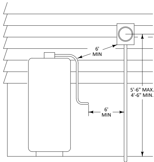
PROPANE GAS
