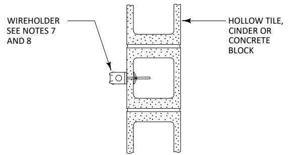
BLOCK
