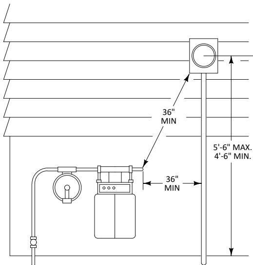
NATURAL GAS
