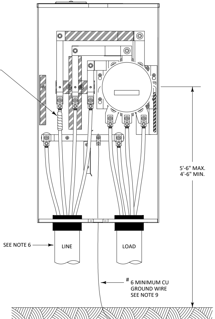
THREE PHASE 4 WIRE 320 AMP SOCKET METER BOX WITH BY-PASS SWITCH SEE NOTES 1 AND 2
