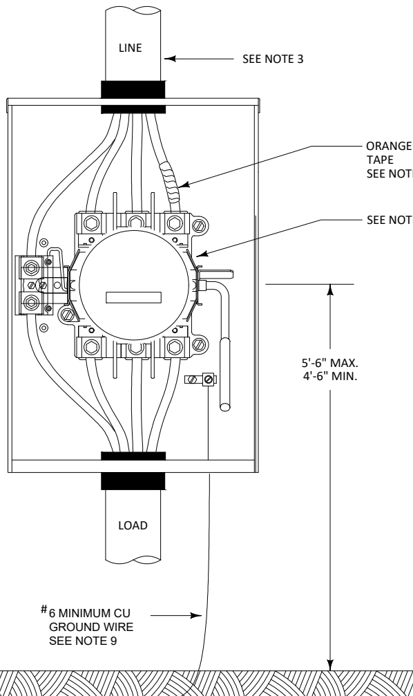
THREE PHASE 4 WIRE 200 AMP SOCKET METER BOX WITH BY-PASS SWITCH SEE NOTES 1 AND 2
