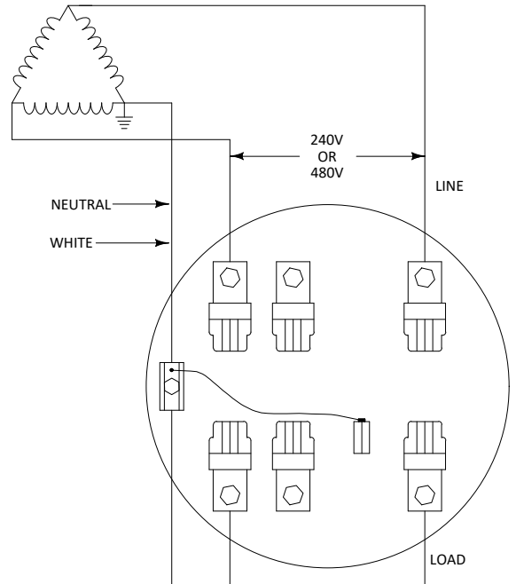
3-WIRE 240 OR 480 VOLT THREE PHASE SELF-CONTAINED 7 TERMINAL SOCKET INDIANA, KENTUCKY, MICHIGAN, OHIO, TENNESSEE, VIRGINIA, WEST VIRGINIA
