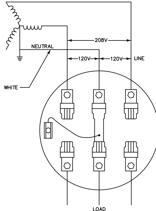
3 WIRE NETWORK 120/208 VOLT SINGLE PHASE SELF CONTAINED
