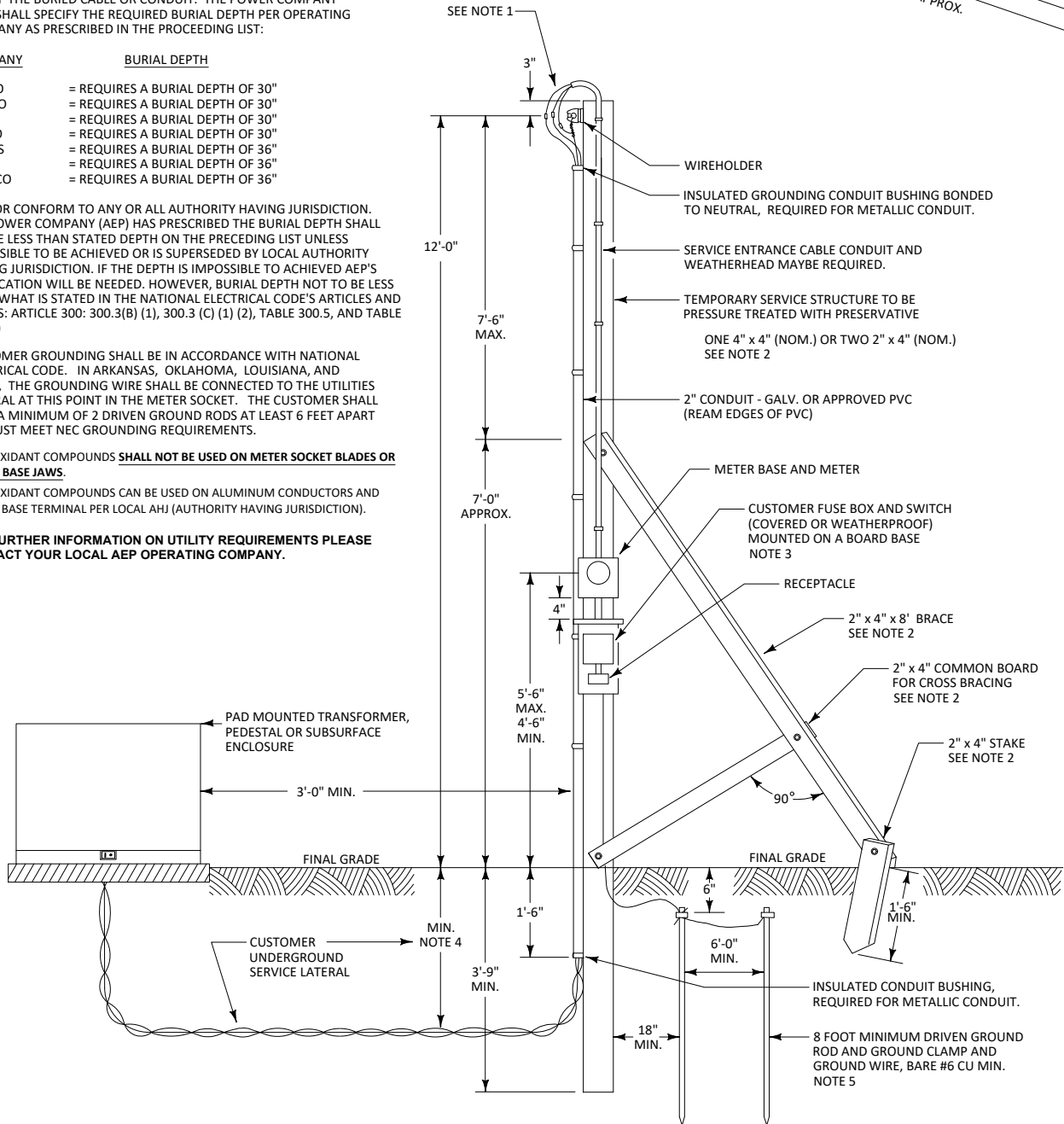
ALTERNATE TEMPORARY SERVICE INSTALLATION FROM EXISTING URD SECONDARY
