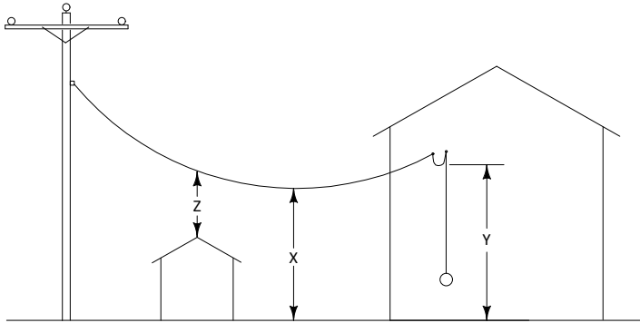
X IN-SPAN GROUND CLEARANCE Y DRIP LOOP GROUND CLEARANCE Z ROOF OR BALCONY CLEARANCE
